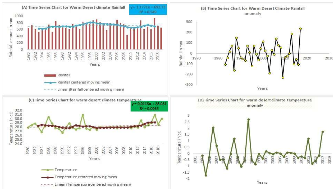
Figure 6: Rainfall and temperature time series and anomaly plots for the Warm Desert Climate Belt.
