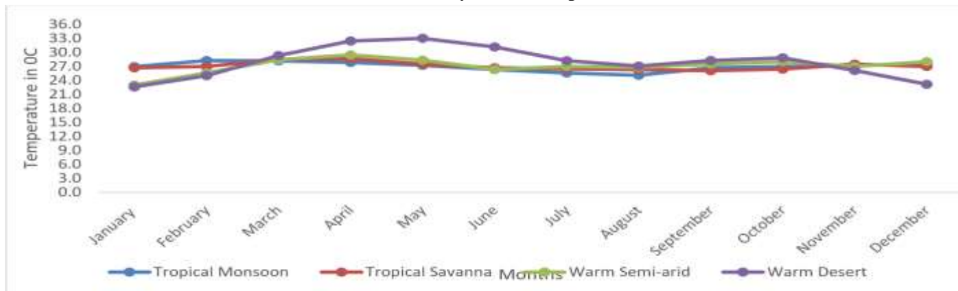
Figure 2: Mean monthly temperature distribution across the climate belts of Nigeria
