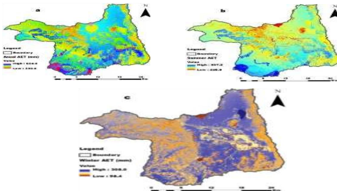
Figure 3. Actual evapotranspiration from Hormat - Golina sub basin.
