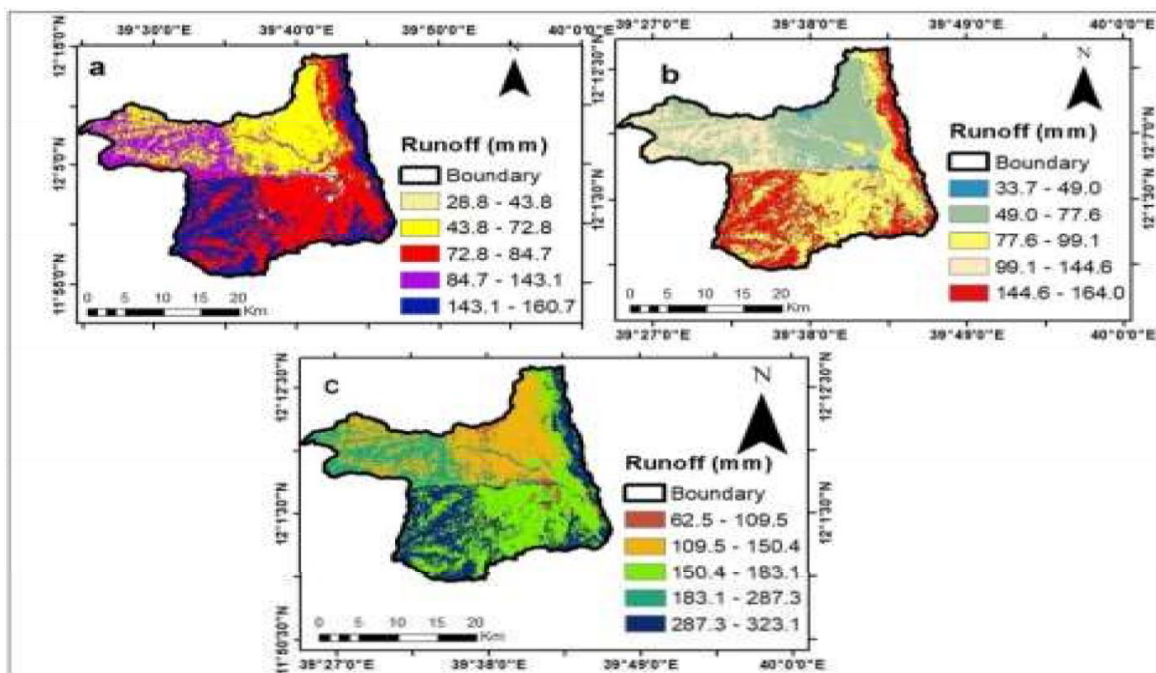
Figure 4. Surface runoff from Hormat -Golina sub basin.
