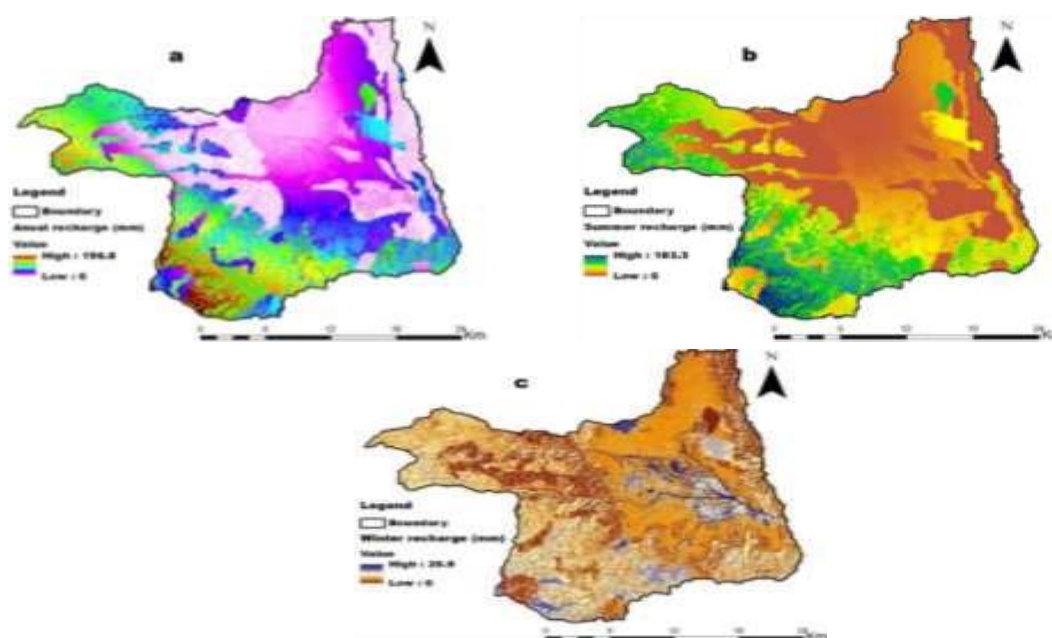
Figure 2. Ground water recharge map of Hormat -Golina sub basin.
