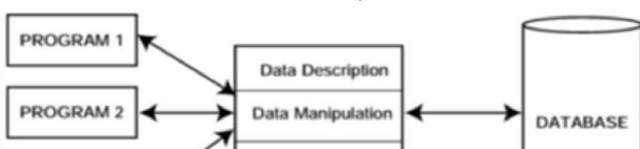
DBMS
