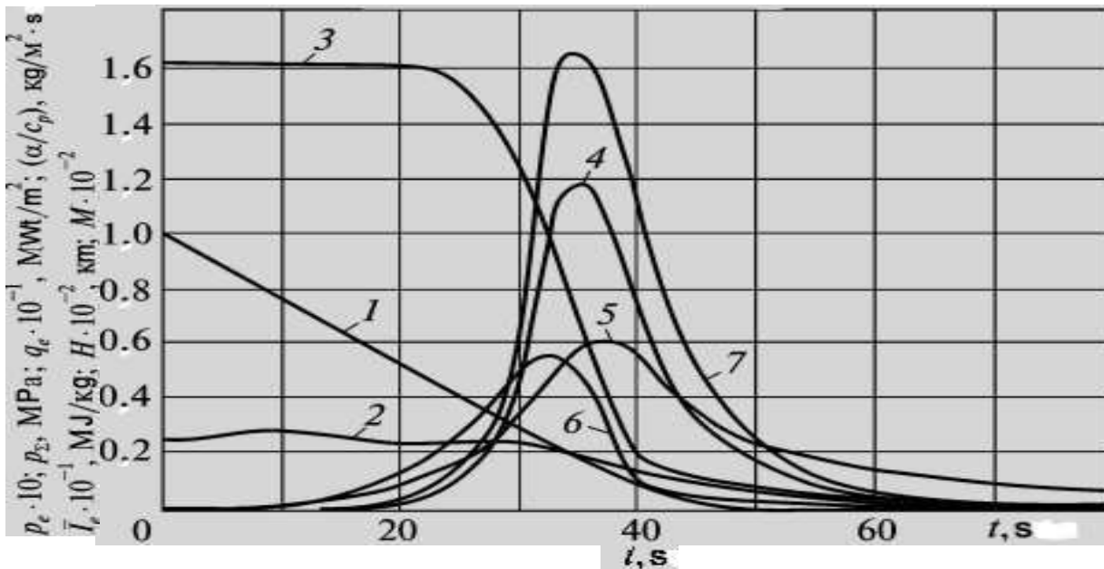
Figure 1. Dependence of parameters of gaseous dynamic flow acting on a side surface of a re-entry spacecraft vs. descent time t from the Earth orbit ( H - 1 ; M - 3 ; I_e - 3 ; p_e - 4 ; \alpha/c_p - 5 ; q_e - 6 ; p_\Sigma - 7 ) [1].
