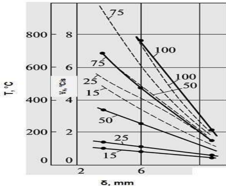
Figure 2. Destruction of surface layers of a thermal shield made of a polymer composite material tested at a high-temperature of gas flow.
