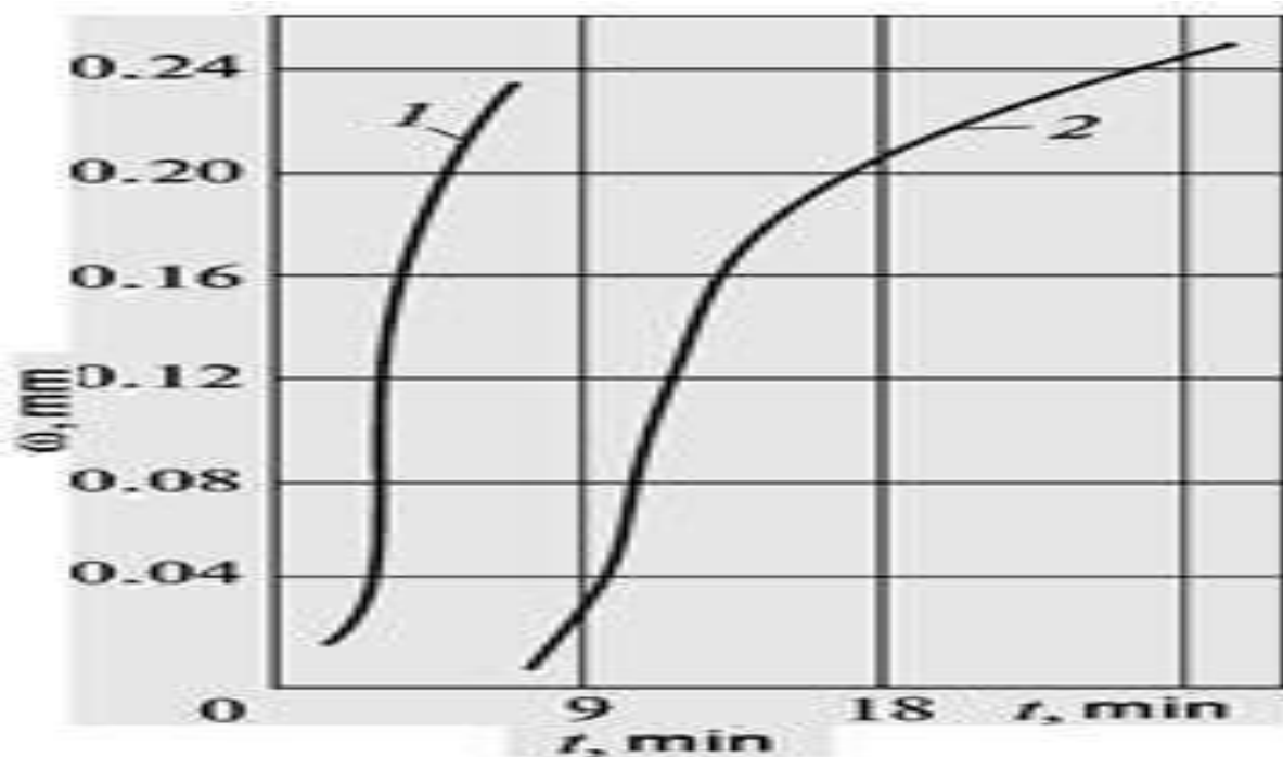
Figure 9. Bending of samples from fiberglass in one-sided heating: 1 – V_h = 100^\circ\text{C}/\text{min} ; 2 – V_h = 25^\circ\text{C}/\text{min} .
