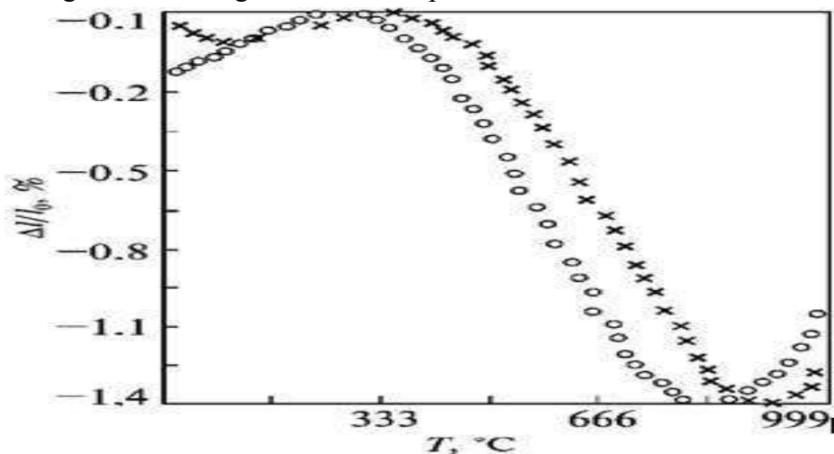
Figure 5. Dependence of relative thermal deformation of glass plastic on temperature (numerical experiment) at heating rates of ^\circ\text{C}/\text{min} , x – 25; o – 75.
