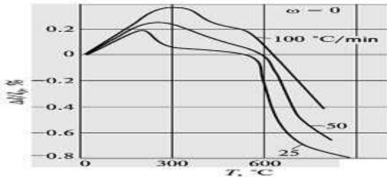
Figure 8. Dependence of the relative deformation of fiberglass TSP-F on temperature in one-sided heating.
