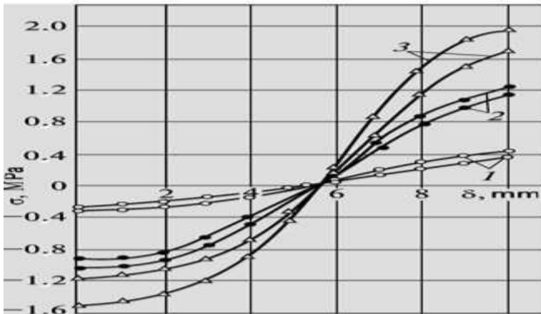
Figure 10. Distribution of stresses in samples from fiberglass in onesided heating: 1 (o) - □ = 1.5 min; 2 (□) - □ = 2 min; 3 (□) - □ = 3 min (continuous curves – straightened sample; non-continuous – bent)
