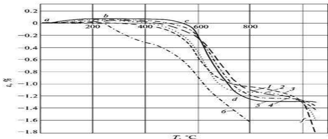
Figure 4. Dependence of the relative thermal deformation of fiberglass TSP-F on temperature at heating rates of °C/min: 1 – 10; 2 – 20; 3 – 25; 4 – 50; 5 – 75; 6 – 5.
