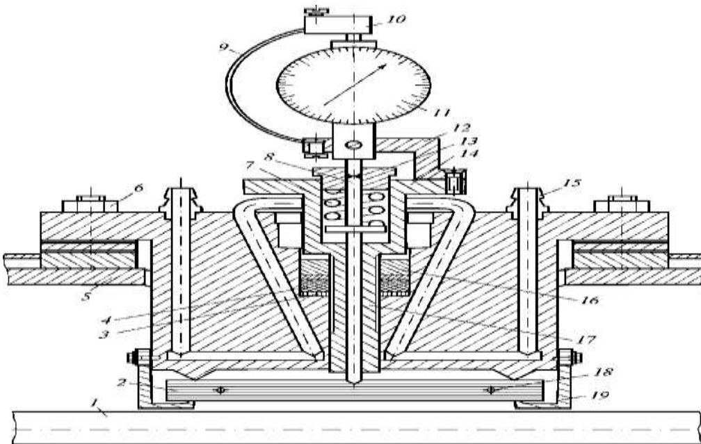
Figure 6. Placement of the sample in a testing chamber under oneside heating: 1 - carborundum heater; 2 - sample; 3 - supporting rings; 4 - rubber rings; 5 - chamber wall; 6 - bolt connection; 7 - spring; 8 - rod; 9 - semi-ring with a tenso-resistor; 10 - clamp; 11 - indicator; 12 - support; 13, 16 - support nuts; 14 - circular platform; 15 - tubulure; 17 - ram; 18 - fiducial; 19 - sample supports.
