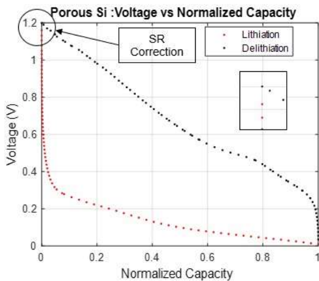
Figure 1a. Voltage vs Normalized Capacity before Side Reaction Correction. Red dots indicate Lithiation and Black dots denote delithiation.
