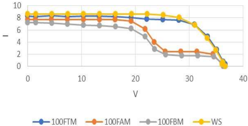
Figure 7. Characteristic of the IV curve of monocrystalline module without shading and with 100% partial shading of the cell by the three materials. Source: results of my work
