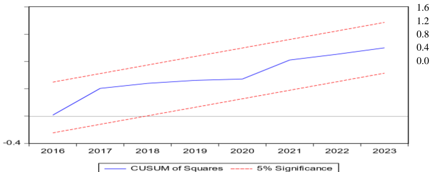
Fig 1: CUSUM of Squares Test
