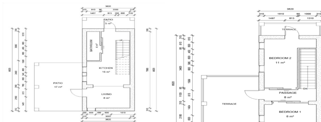
Figure 5: A 10X10 Sandbag House floor plans
