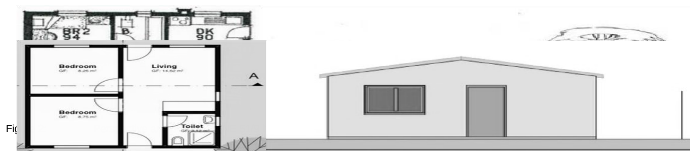
Figure 3: Plan and elevation of a typical 40m 2 RDP house
