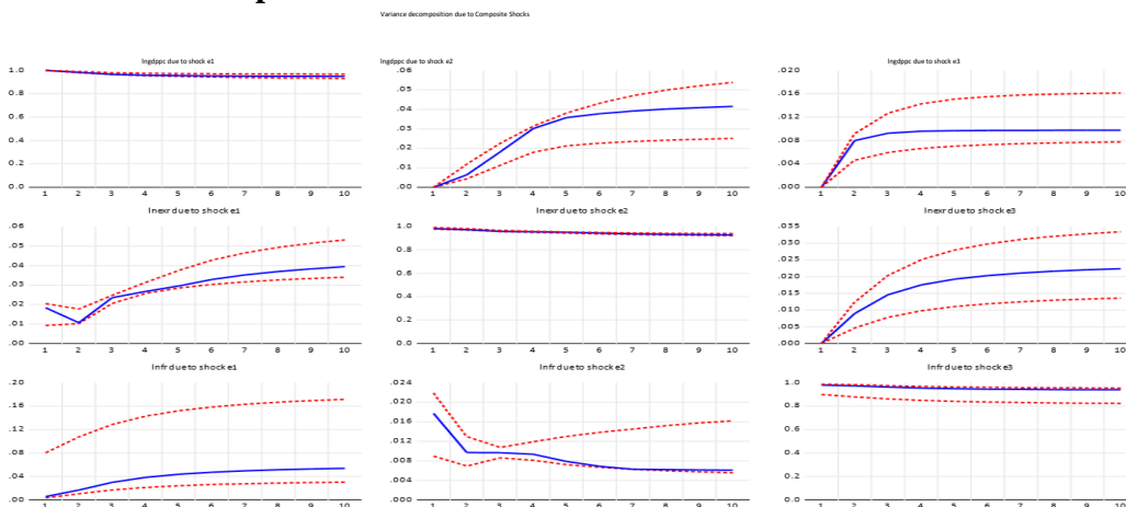
Figure 3.14: Plots of Variance Decomposition due to composite shock
