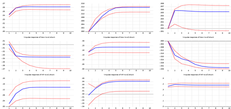
Figure 3.13: Plots of Impulse Response due to idiosyncratic Variance Decomposition
