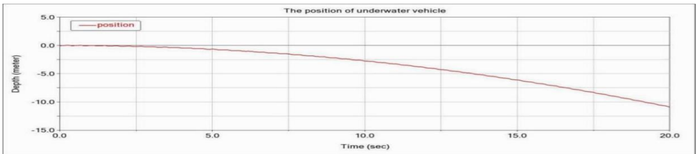
Figure 4: The relationship between the position of AUV's center of mass and time when AUV ascent.
