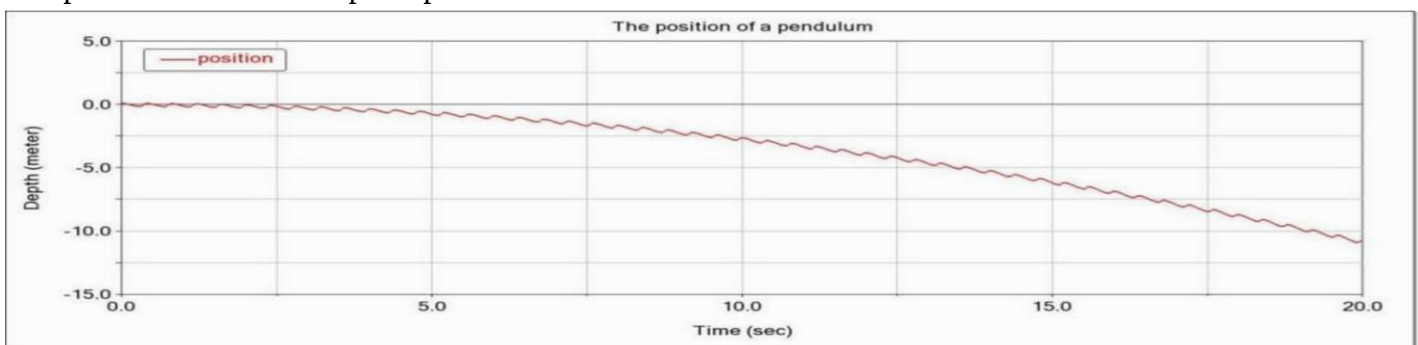
Figure 6: The relationship between pendulum's position and time when AUV ascent.
