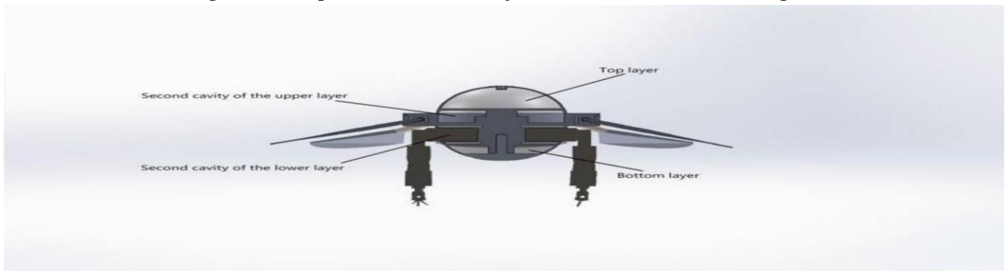
Figure 3: Section view of the octopus-like AUV.
