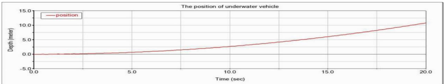
Figure 7: The relationship between the position of AUV's center of mass and time when AUV descent.
