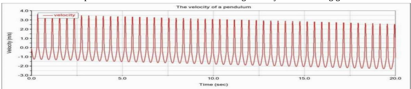
Figure 5: The relationship between pendulum's velocity and time when AUV ascent.
