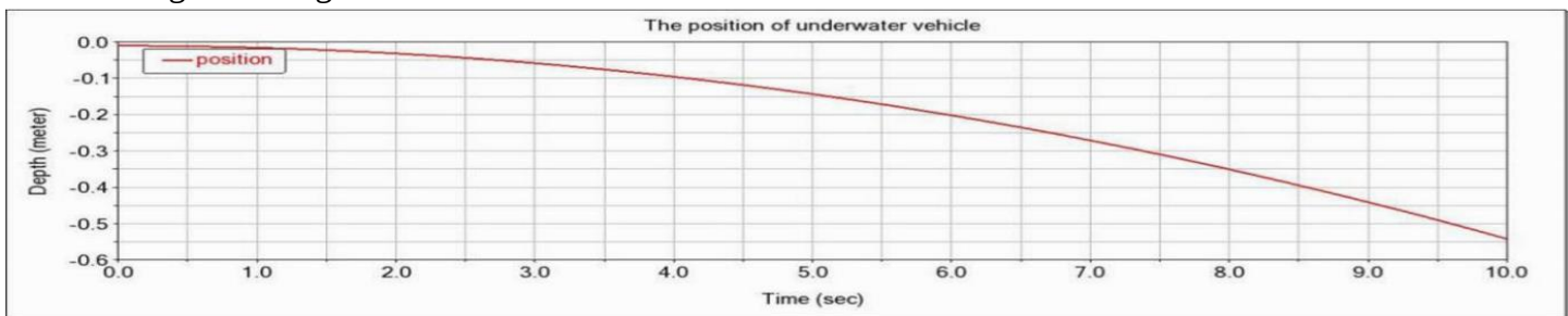
Figure 14: The change of the position of the center of mass in the first 10 seconds when eight pendulums flap simultaneously.
