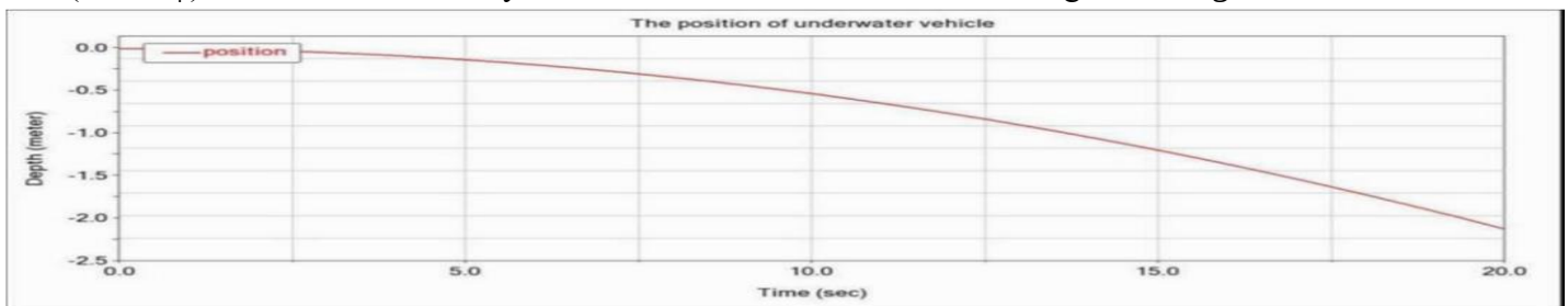
Figure 11: The relationship between the position of AUV's center of mass and time for harmonic motion.
