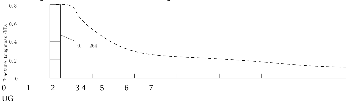
Figure 1: Changing Law of Rock Fracture Toughness
