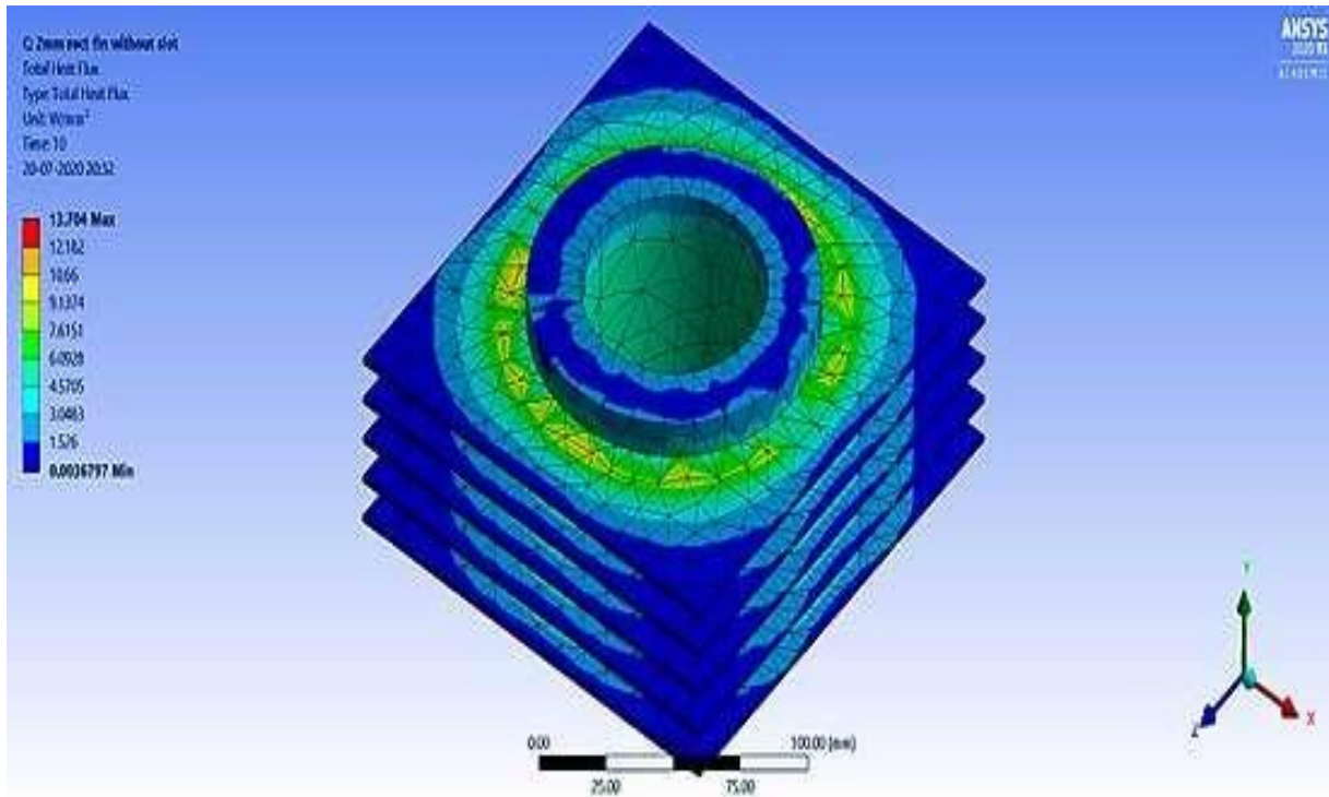
Figure 18. Total heat transfer per unit area in rectangular fin 2 mm without slot.
