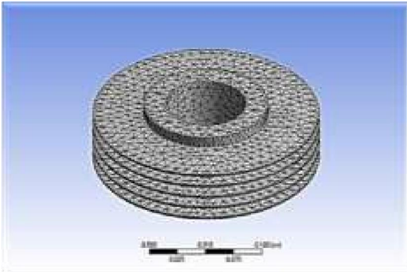
Figure 8. Mesh model of circular fin.
