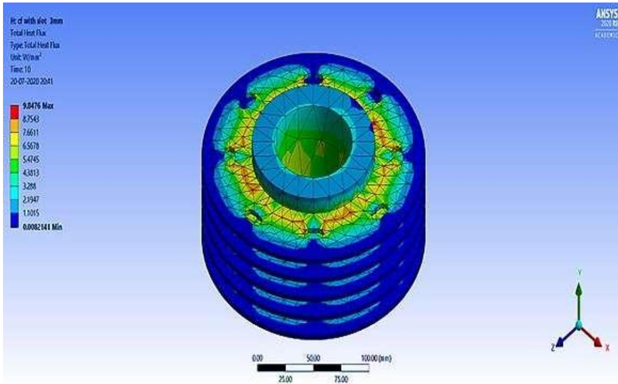
Figure 25. Total heat transfer per unit area in circular fin 3 mm with slot.
