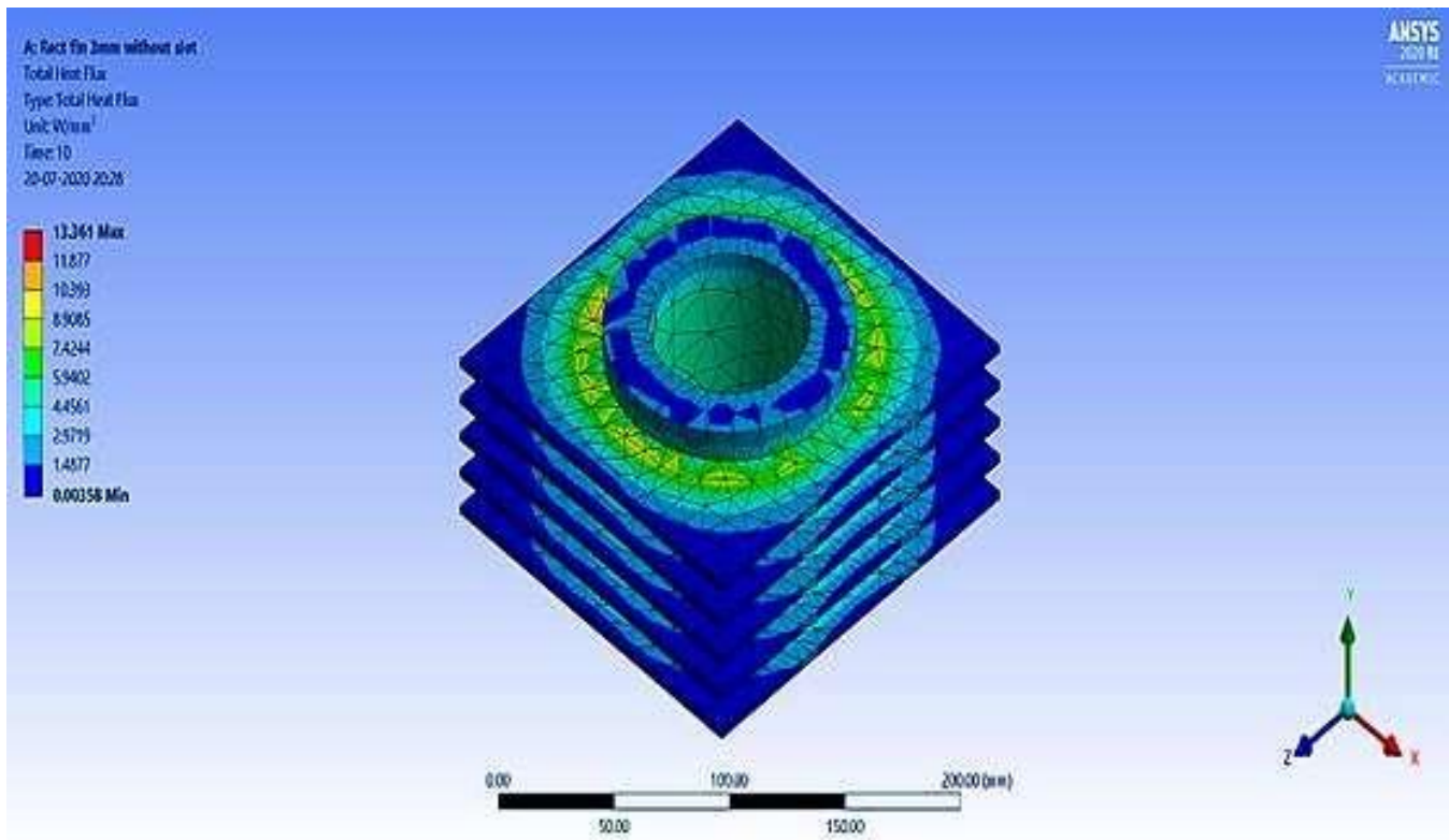
Figure 20. Total heat transfer per unit area in rectangular fin 3 mm without slot.
