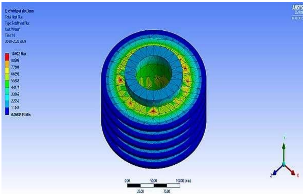
Figure 24. Total heat transfer per unit area in circular fin 3 mm without slot.
