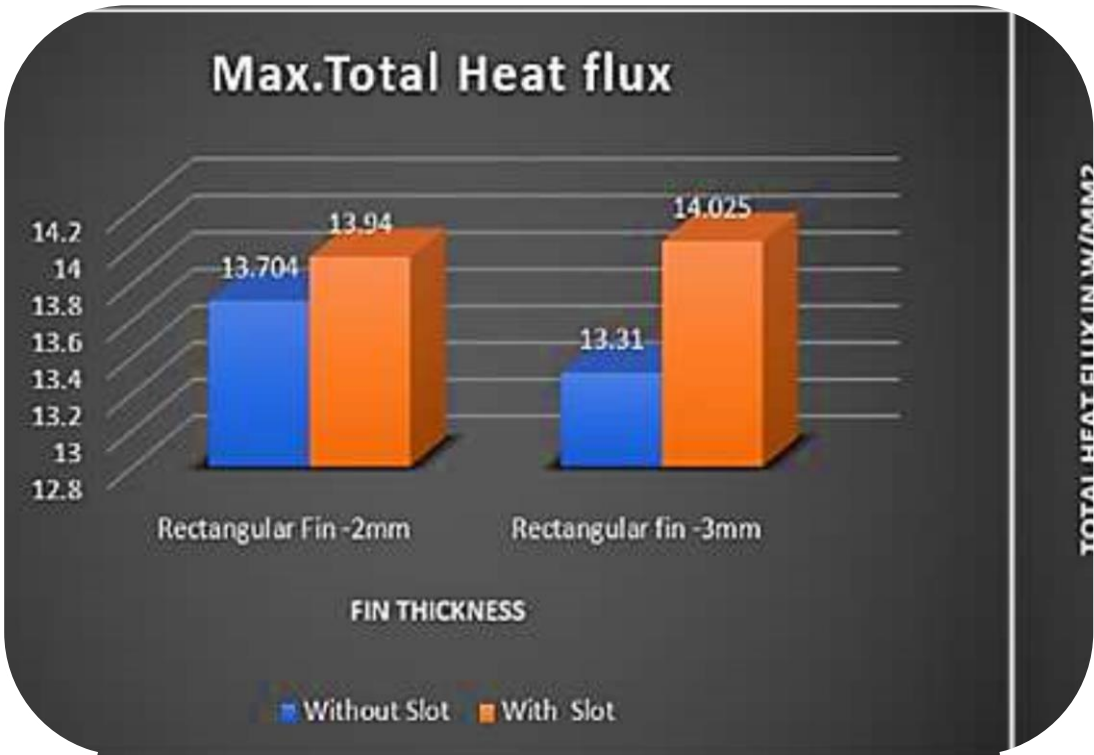
Figure 28. Total heat transfer per unit area in rectangular fins of varying thickness.
