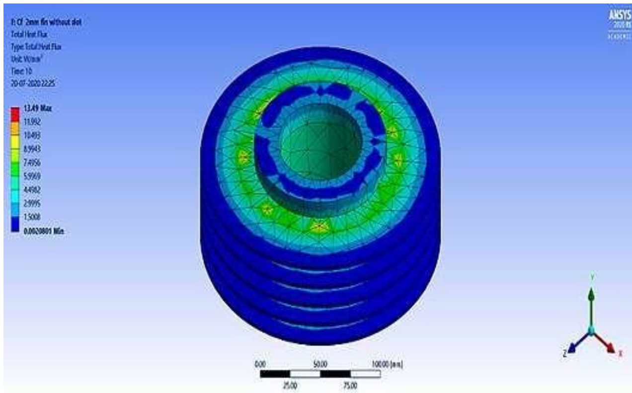
Figure 22. Total heat transfer per unit area in circular fin 2 mm without slot.
