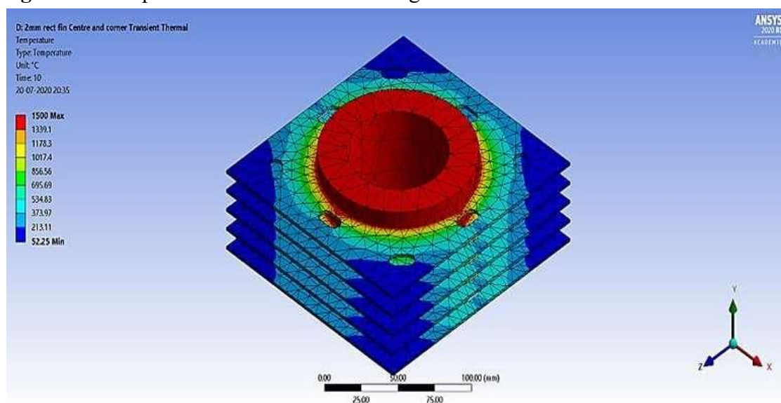
Figure 11. Temperature distribution in rectangular fin 2 mm thick with slot.
