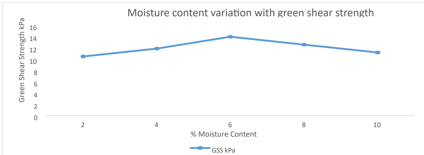
Figure 1: Moisture Content Variation with Green Shear Strength
