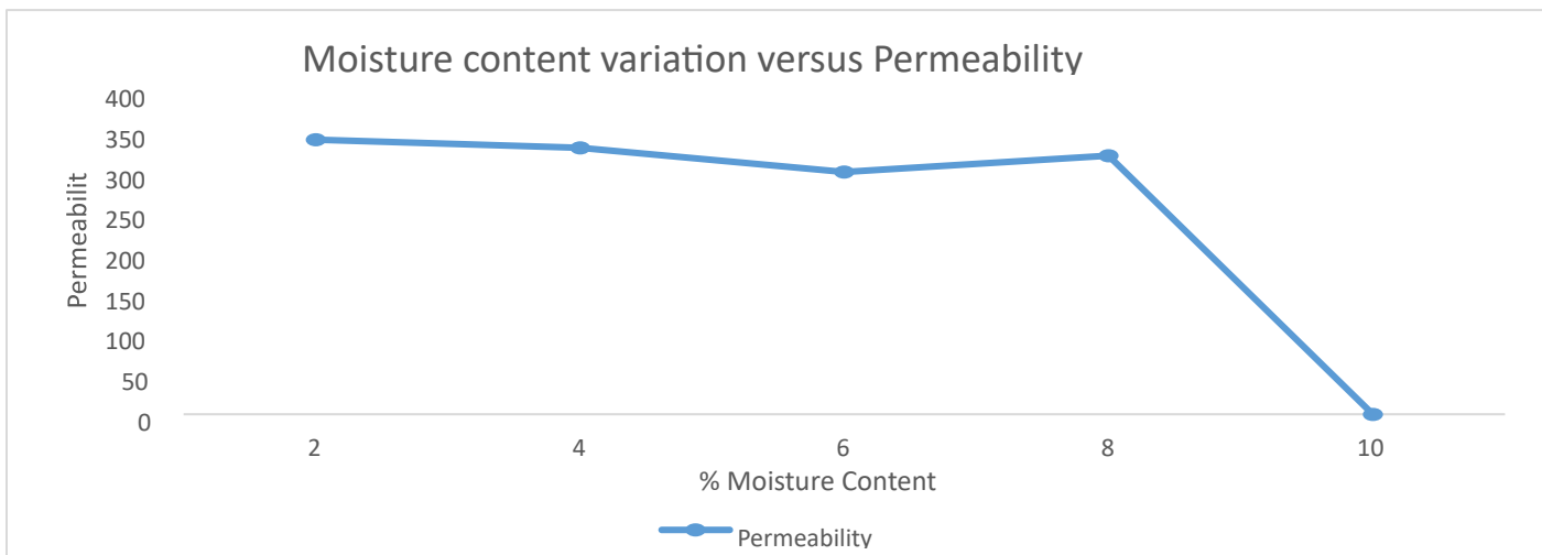
Figure 3: Moisture variation with Green Permeability of Use Offot Sand
