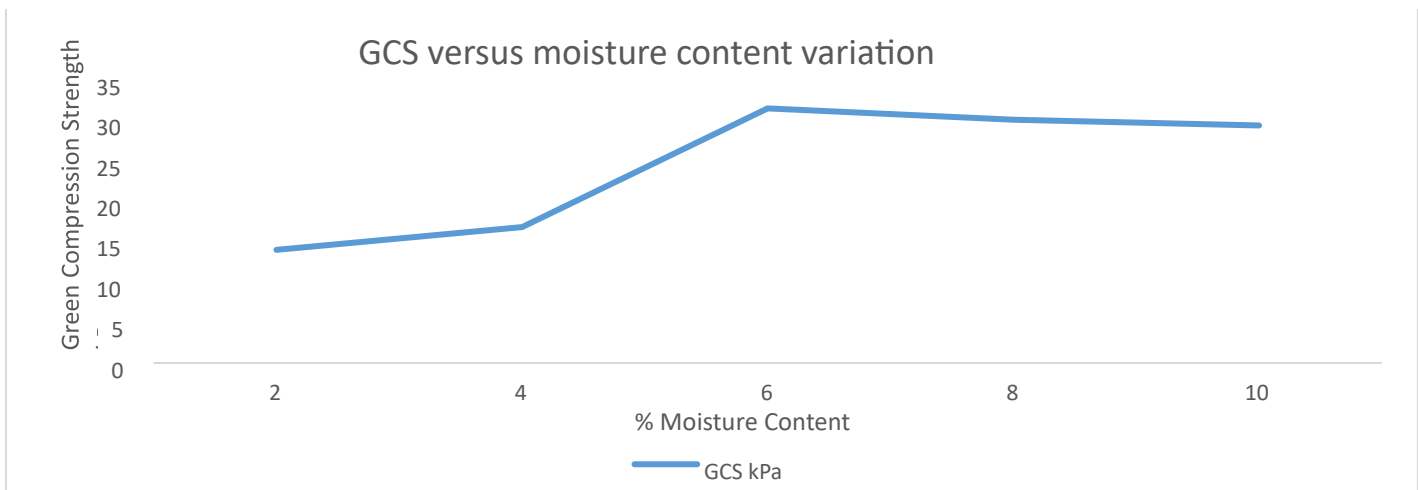
Figure 2: Moisture content variation with Green Compression Strength of Use Offot Sand
