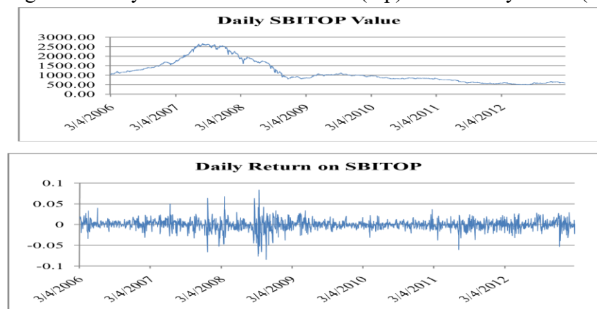
Figure 1: Daily value of SBITOP index (top) and its daily return (bottom)
