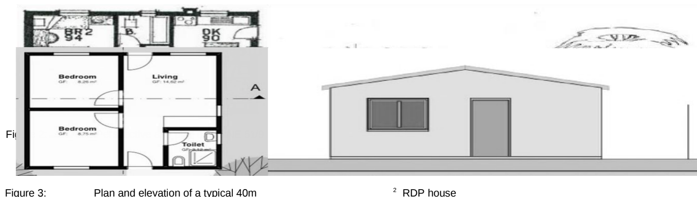
Figure 3: Plan and elevation of a typical 40m
