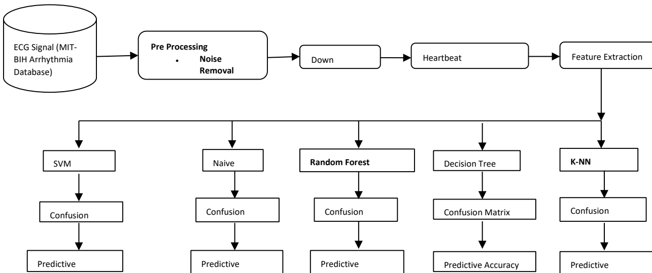
Figure 2. Proposed arrhythmia classification system
