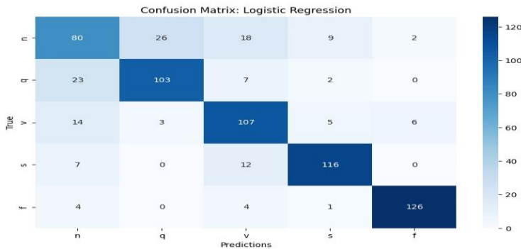
Figure 13: Confusion matrix of the Logistic Regression
