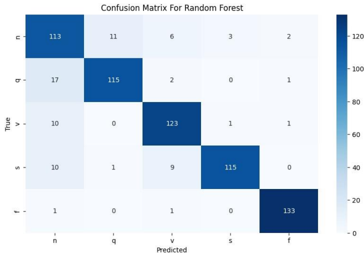
Figure 9: Confusion matrix of the Random Forest Model
