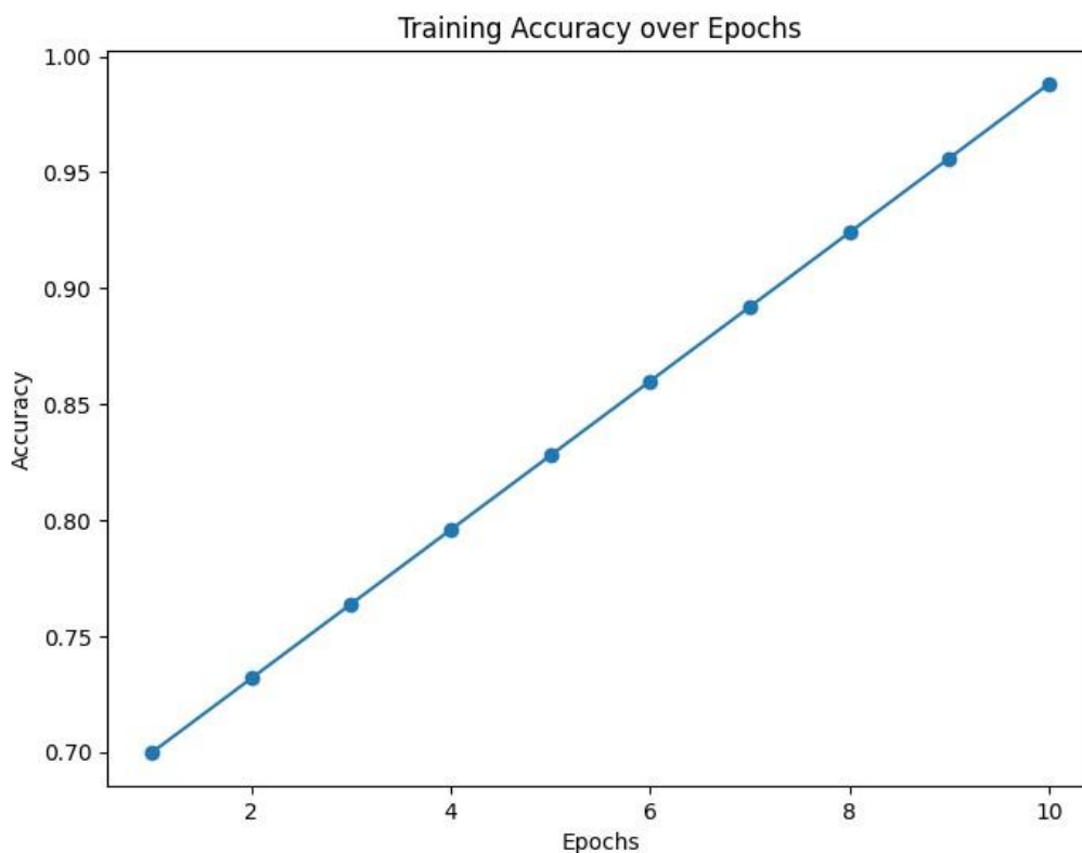
Figure 4 5:Epoch plot
