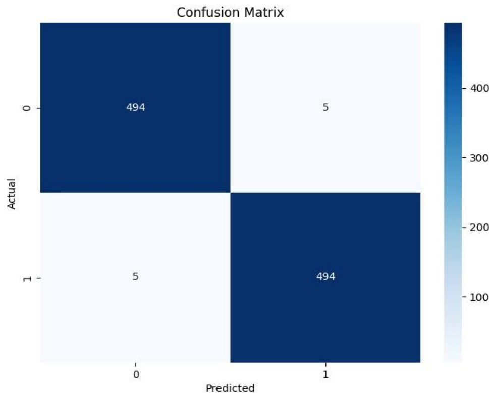
Figure 4 4:ConfusionMatrix
