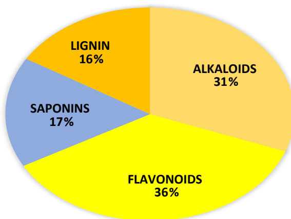
FIG. 1: some antioxidant compounds present in dried banana peels
