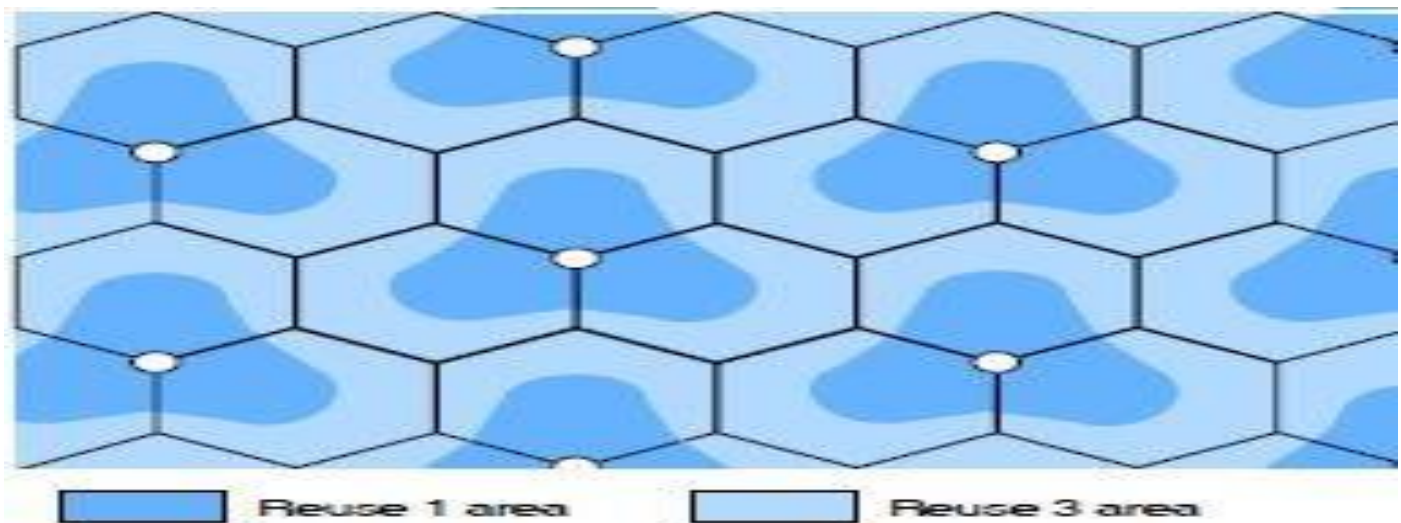
Figure 4: Illustration of Fractional Frequency Reuse with two reuse.
