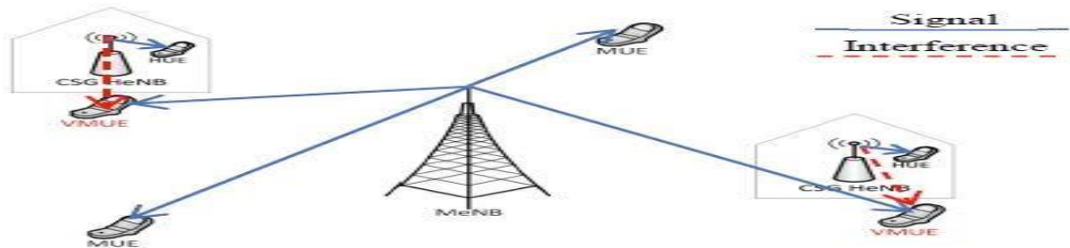
Figure 1: HetNet Environment.
