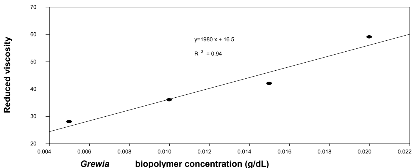
Figure 4. Huggin's plot of Grewia spp. Biopolymer.
