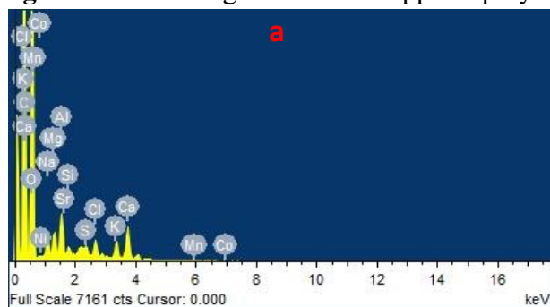
8. Energy dispersive spectroscopy pattern of Grewia spp. biopolymer before (a) and after purification (b).
