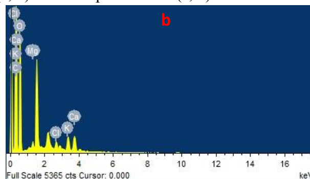
8. Energy dispersive spectroscopy pattern of Grewia spp. biopolymer before (a) and after purification (b).
