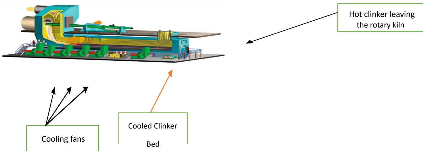
Figure 2. Pictorial view of Clinker Inlet and Clinker cooling. Source: FLSmidth (2015).
