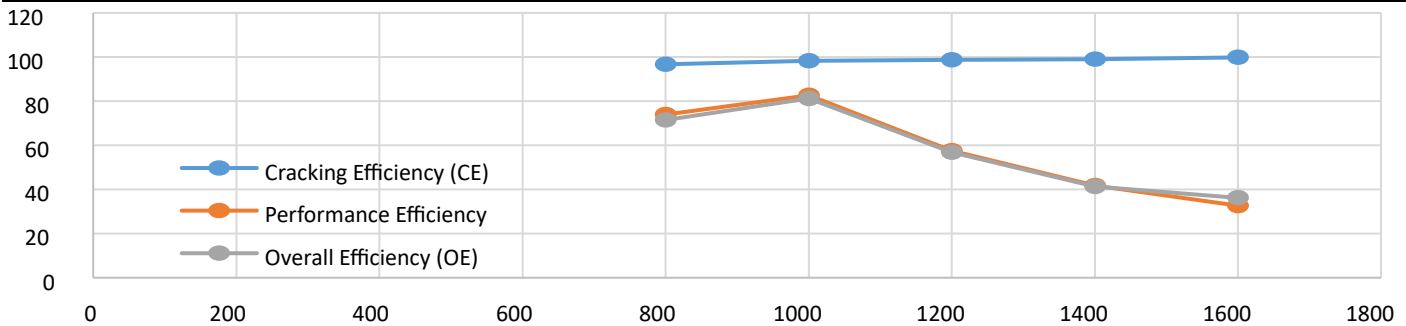
Figure 3.2 Graph of machine efficiencies against speed when the machine is assembled with four arm hammer beaters
