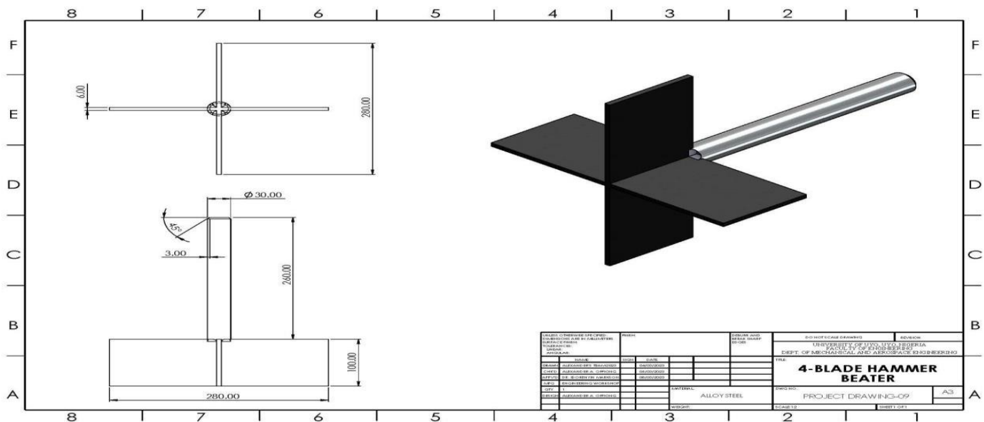
Figure 2:3 Components drawing showing Four Blade Hammer Shaft or Beater Shaft Head
