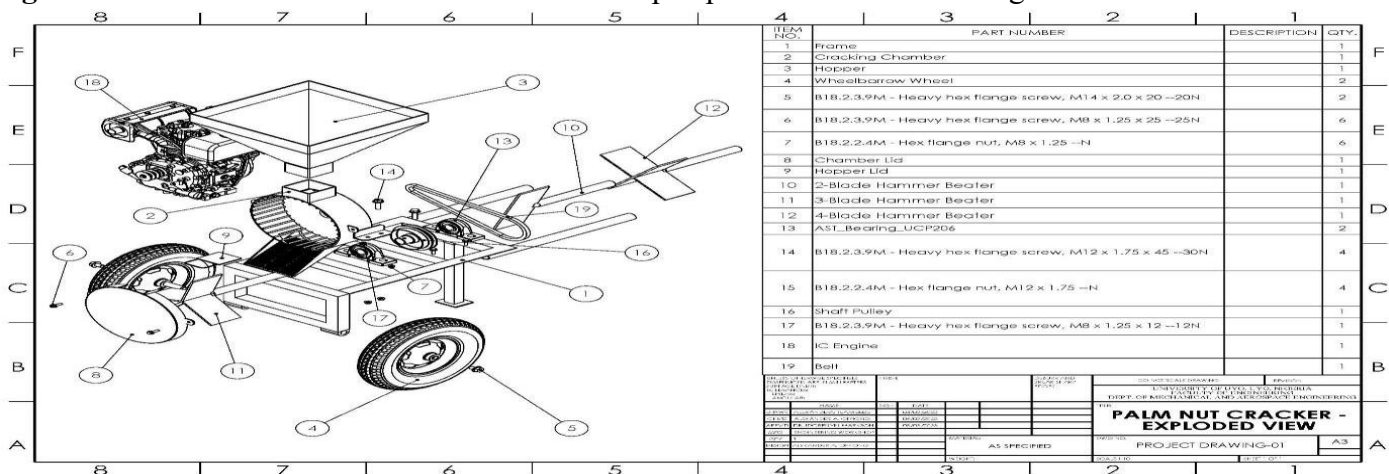
Figure 2.2: Exploded view of model components of the developed palm kernel nut cracking machine
