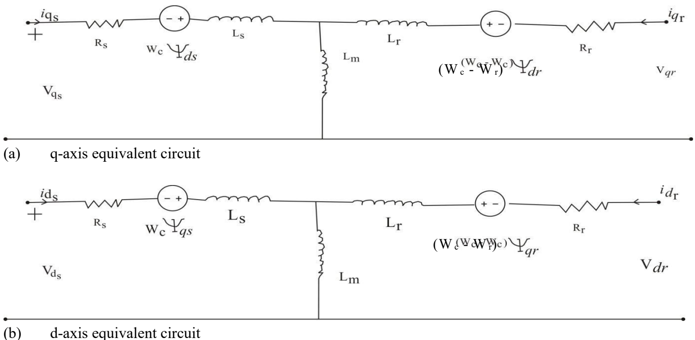
Figure 1: d-q equivalent circuit of the induction motor
