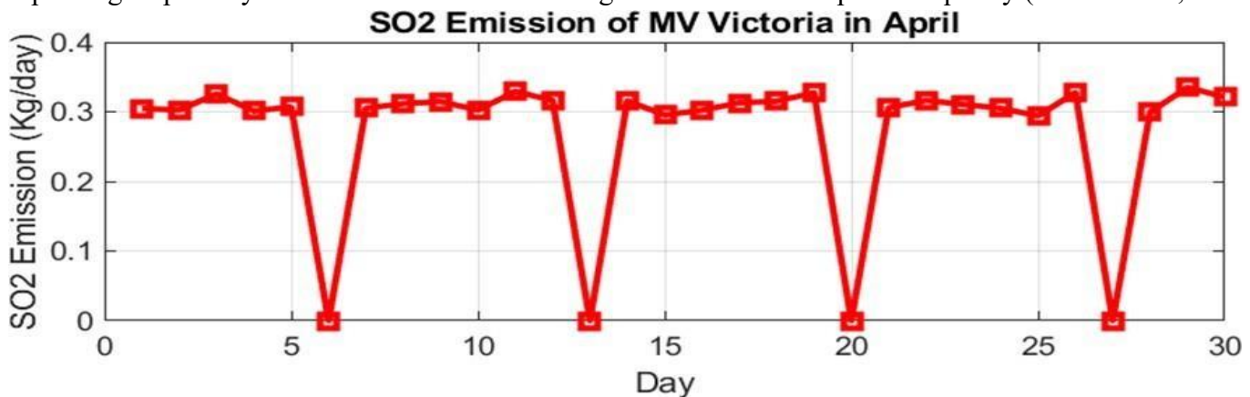
Figure 4.3: Rates of SO2 Emissions
