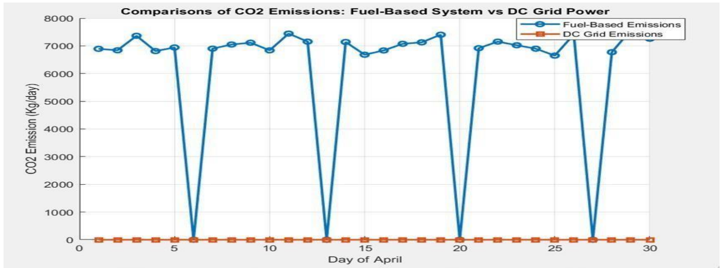
Figure 4.2: Comparisons of CO2 Emissions Between diesel-based vessel and Electric DC grid DC grid system
