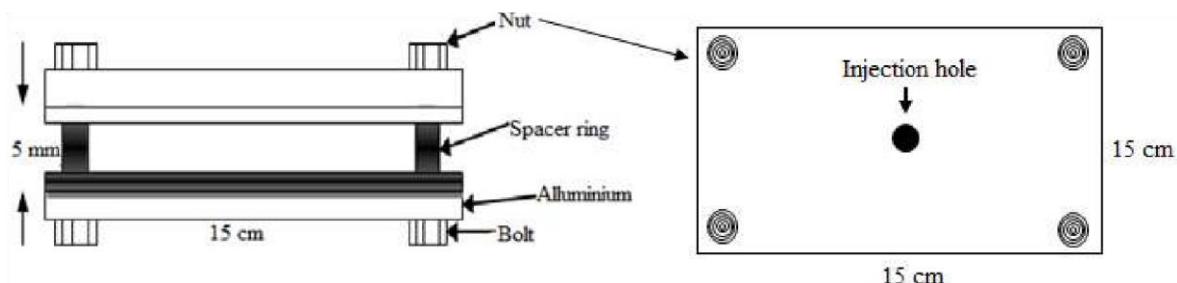
Figure 1. Dimensions of the metallic mold chamber used in this study. Molten RHA-MA-HDPE was injected through the injection hole.
