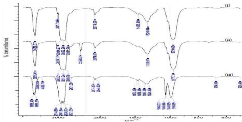
Figure 9. FTIR spectra for oRHA-MA-HDPE (recycled) composites (i) 5 % oRHA (ii) 10% oRHA and (iii) 35 % oRHA.
