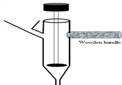
Figure 2. Plunger for injecting molten HDPE-MA-RHA mixture.
