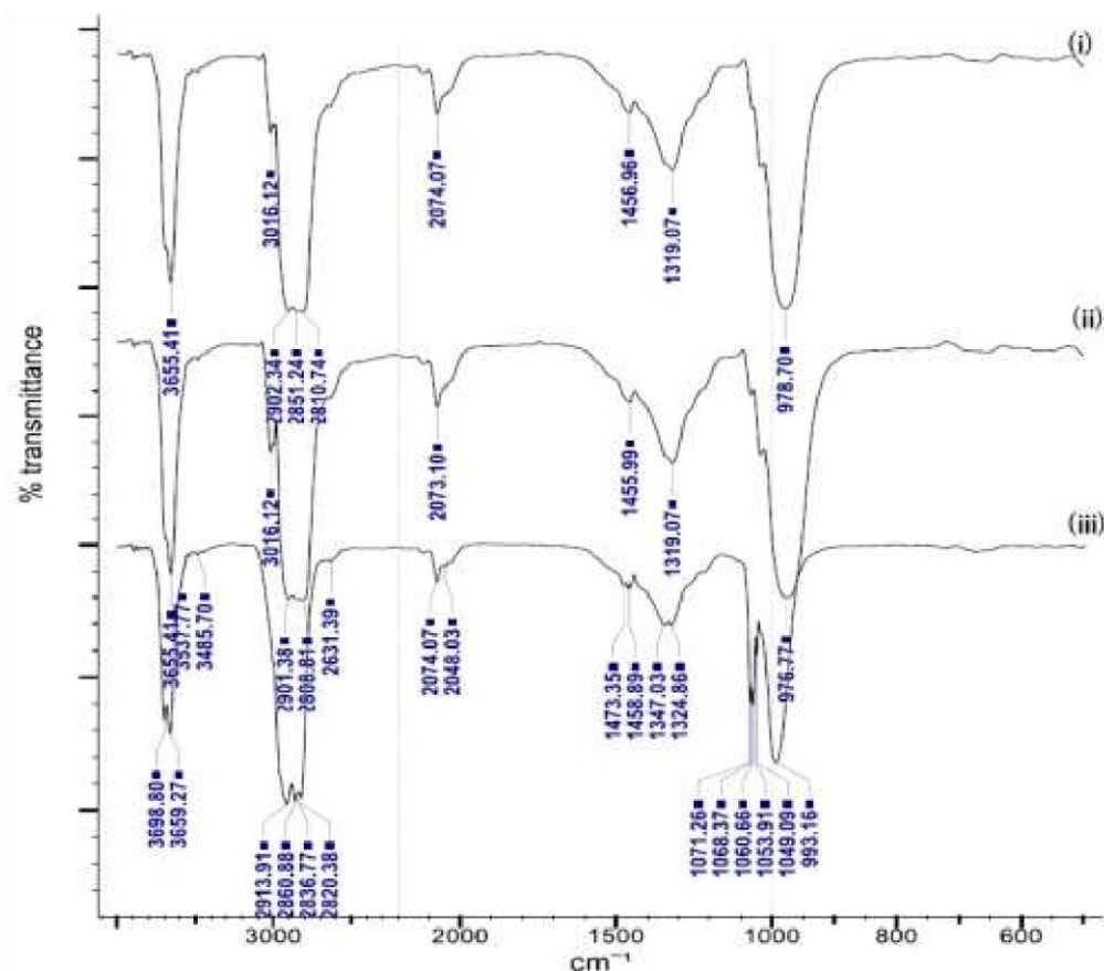
Figure 6. FTR spectra for fRHA-MA-HDPE (pure) composites (i) 5 % fRHA (ii) 10% fRHA and (ii) 35 % fRHA.
