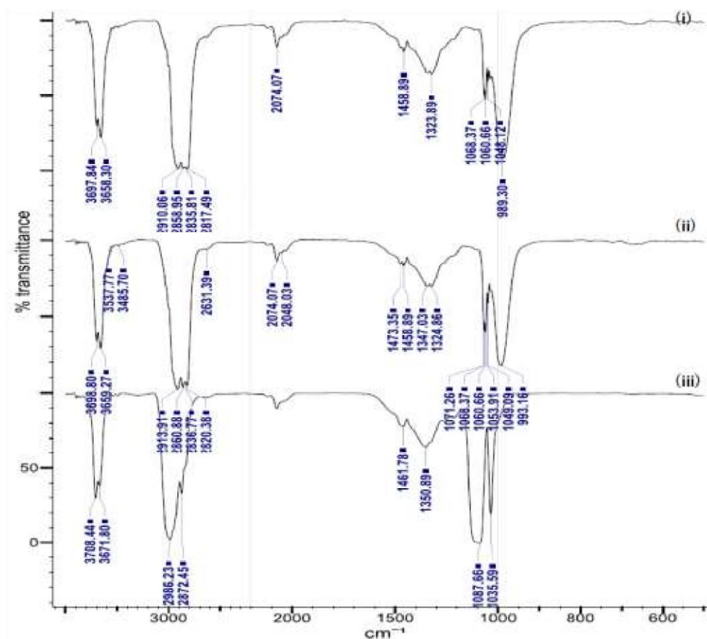
Figure 7. FTR spectra for oRHA-MA-HDPE (pure) composites (i) 5 % oRHA (ii) 10% oRHA and (iii) 35 % oRHA.
