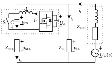
Figure 1: Single-phase ES system connection diagram.
