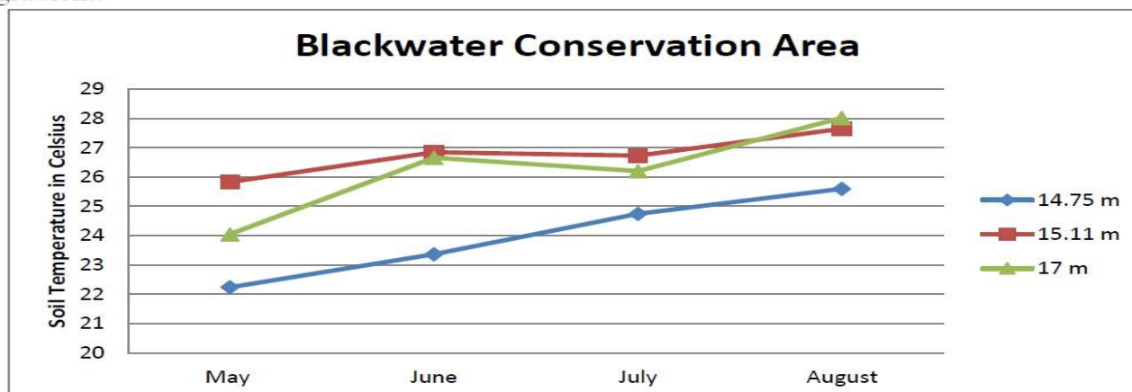
Figure 3. Soil temperature in the bottomland (14.75 m) is consistently lower than the upland (17 m) and Shrub/scrub (15.11) areas. The upland and shrub/scrub areas soil temperatures alternate positions in July and August.
