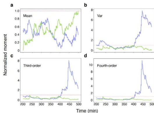
Figure 6: Sensitivity of moments against anomaly. The anomaly occurs at time t = 401 . All the moments are normalized for visual convenience, and the normalization methods are stated in Appendix
